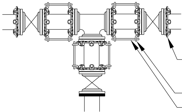
FITTING WITH TIE-RODS AND RESTRAINED JOINT GLANDS
